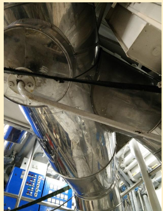
INOX STEEL METAL PLATING AT EXHAUST PIPE IN MAIN ENGINE WITH INSPECTION DOOR
